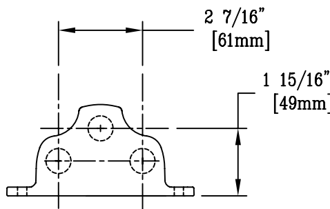
B-0502 Double Pedal Valve
