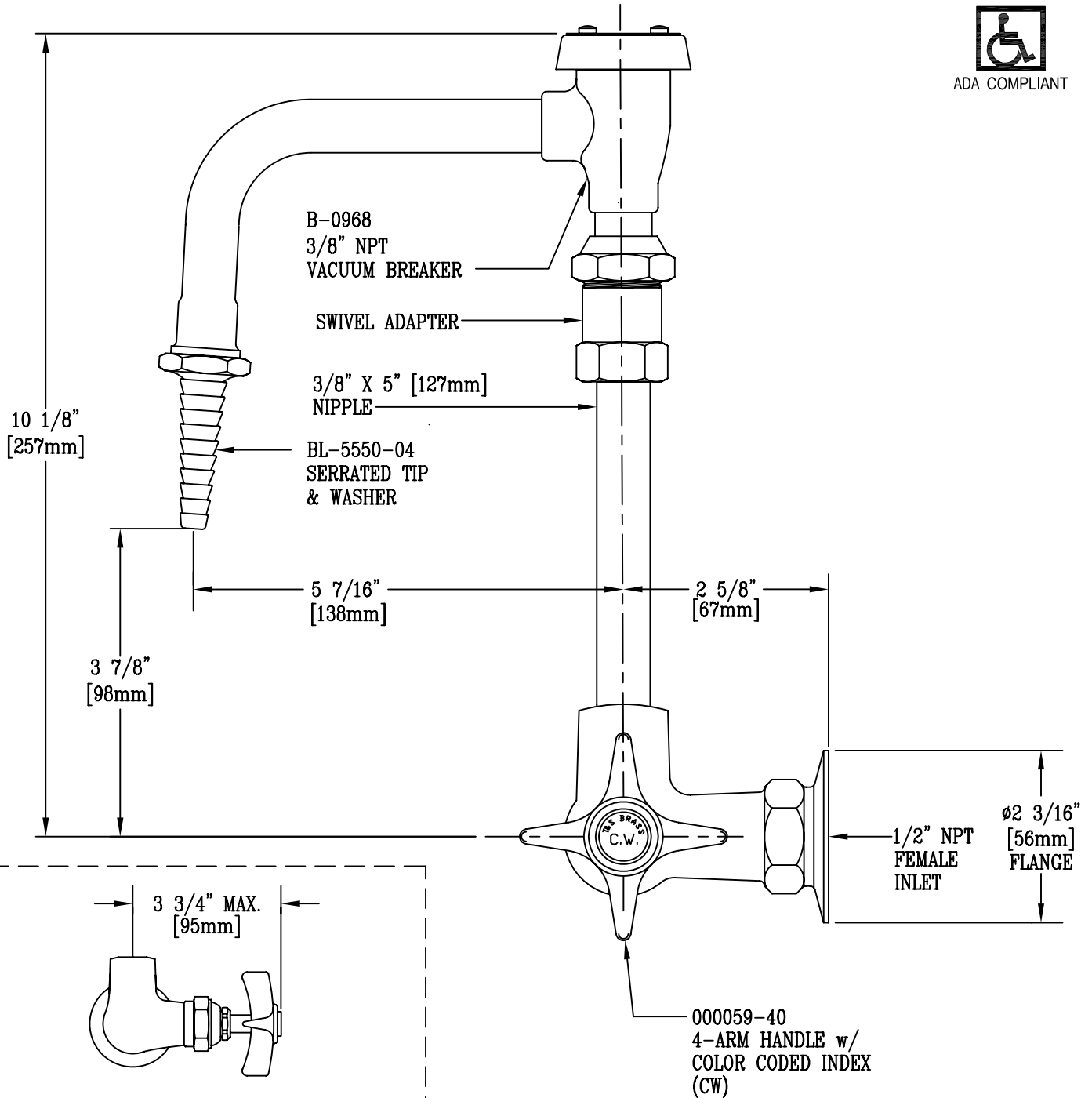
SIDE VIEW - HALF SIZE
