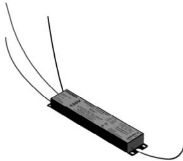
Ballast 800563 QT1X32/120/IS-SCA
