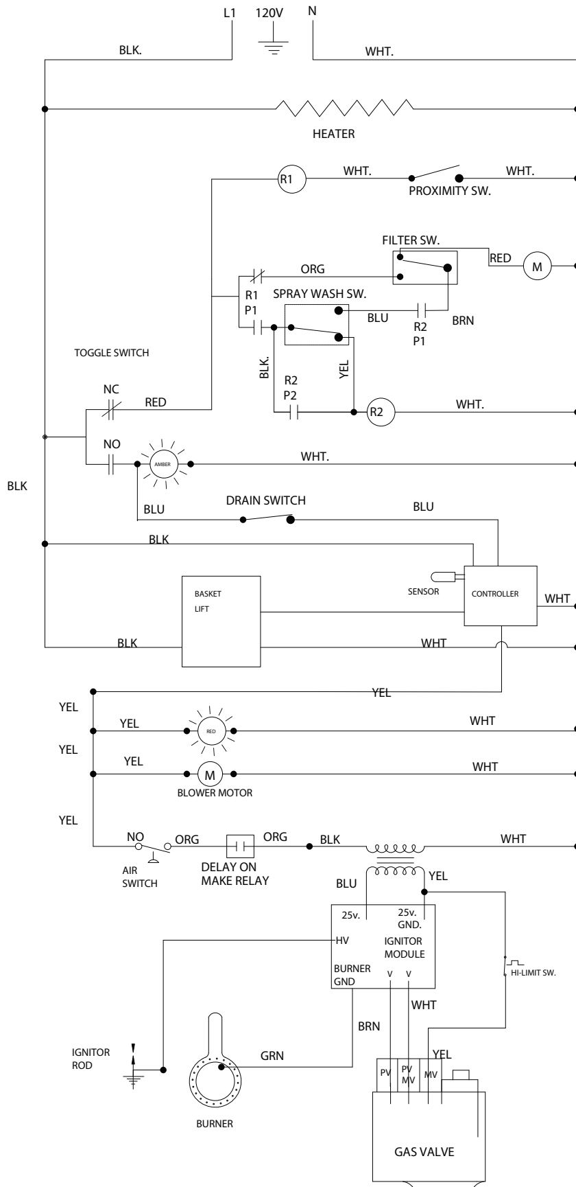
PAR-3-F GAS FRYER WITH COMPUTER WIRING DIAGRAM
