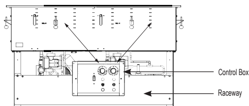
Figure 4. Two well drop-in control box mounting
