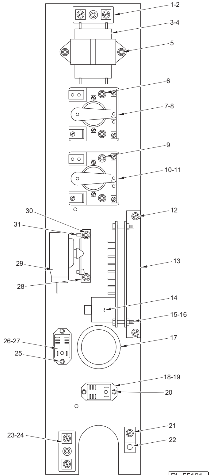
HGC5 / DGC5 (W/COOK & HOLD) ELECTRICAL COMPONENT PANEL
