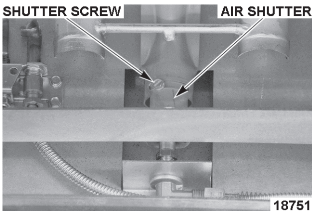
Oven Burner Air Shutter Shown
