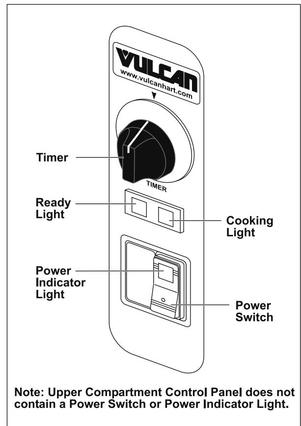
Figure 4. Cabinet Controls
