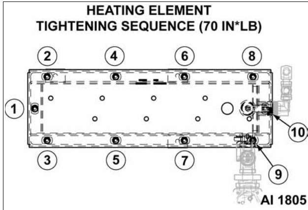
OVERHEAD VIEW OF HEATING ELEMENT
