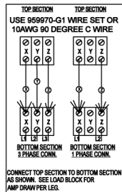
VC3ED 208-240V Wire Diagram
