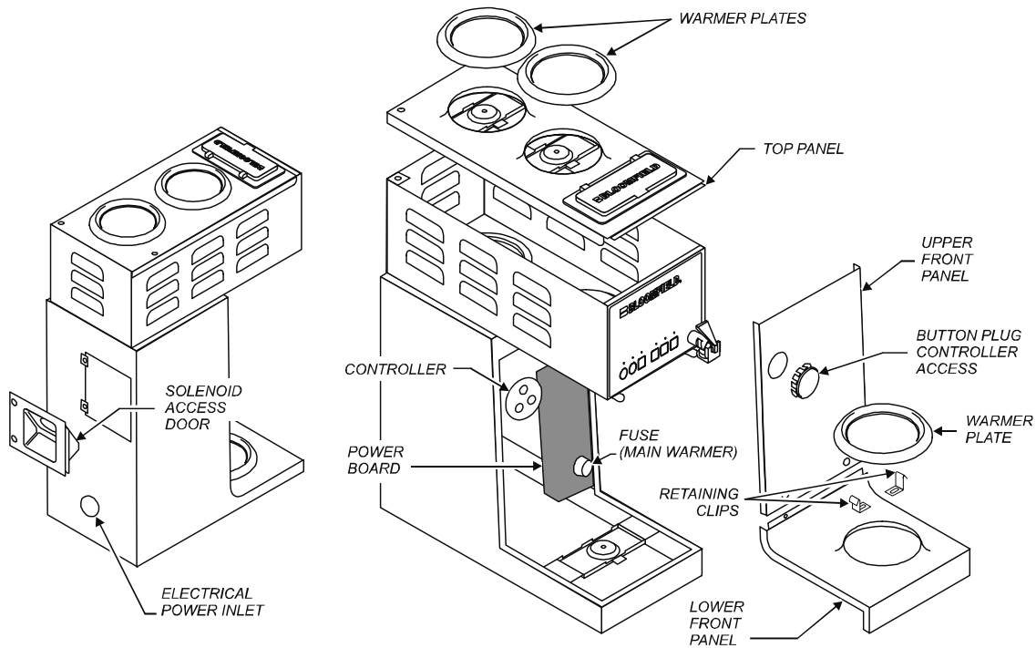
Fig. 12 Access Panels
