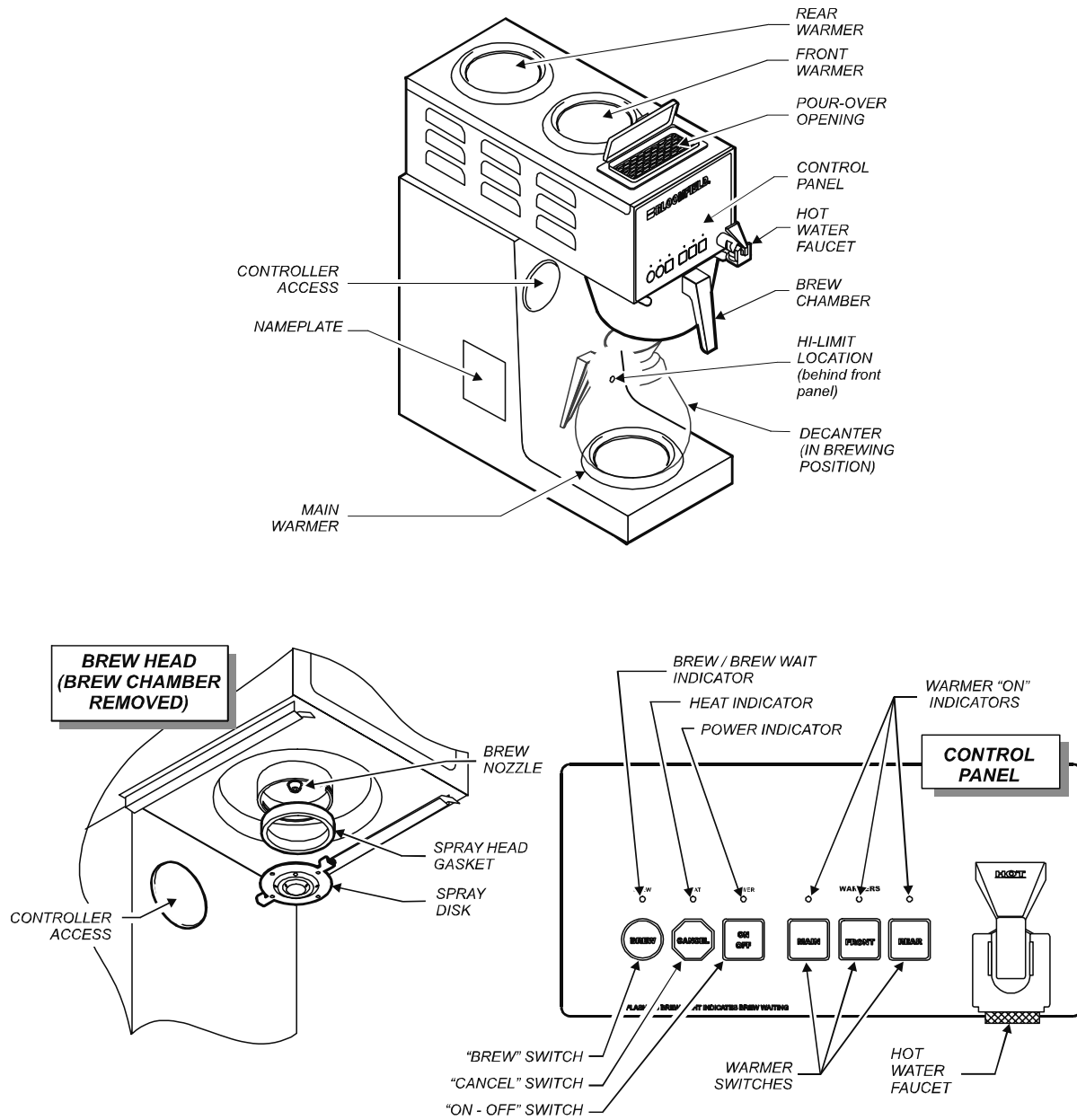
Fig. 1 1016 Features and Operating Controls
