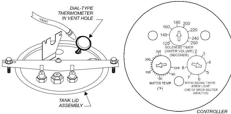
Fig. 13 Checking and Adjusting Brew Temperature
