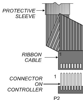
Fig. 18 Keypad Ribbon Cable Hook-Up
