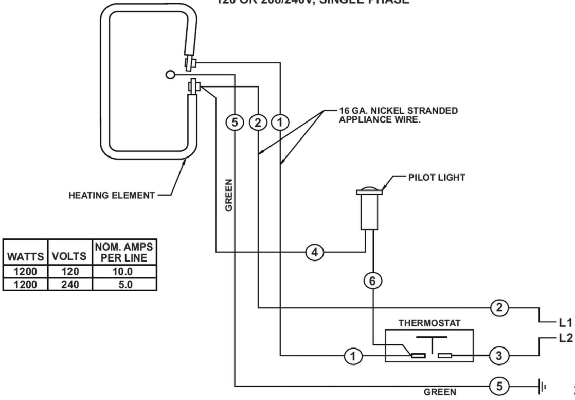
WIRING DIAGRAM FOR SS206T, SS206ET 120 OR 208/240V, SINGLE PHASE
